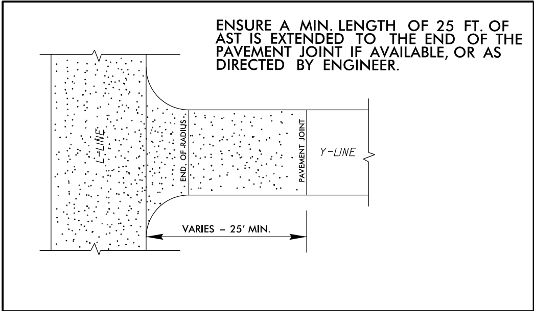
DETAIL 1
